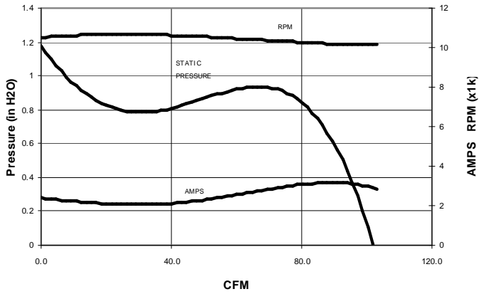
3" Blower Model Series 277-3XXX 12 VDC
