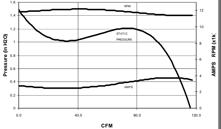
3" Blower Model Series 277-3XXX 13.6 VDC
